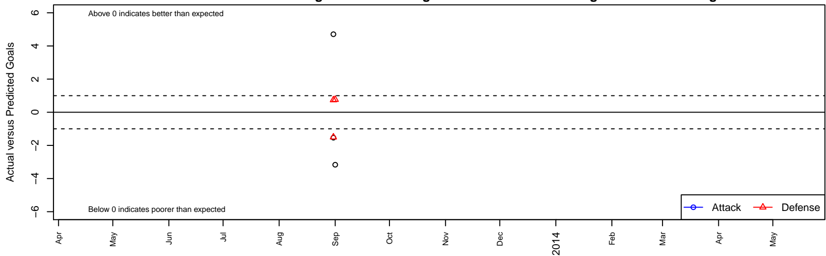
MVP Rapids –Unk B02 Dots are actual minus expected GF (blue circles) and GA (red triangles). Blue line is smoothed change in attack strength. Red is smoothed change in defense strength.
